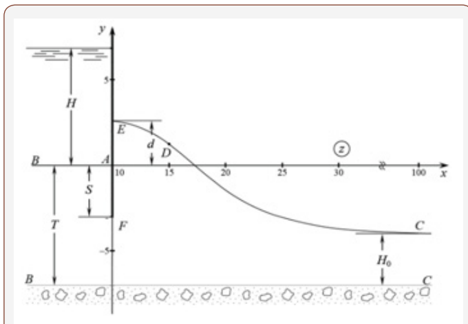
Figure 1(a): The current picture calculated at \epsilon = 0.6 , h_c = 0.5 , T = 7 , S = 3 , H = 5 .
