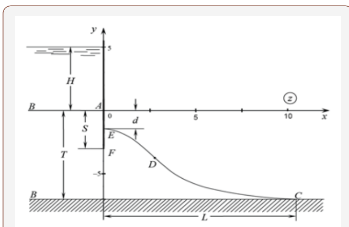
Figure 1(b): The current picture calculated at \epsilon = 0.6 , T = 7 , S = 3 , H = 7 , H_0 = 3 и x_C = 100 .
