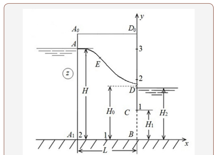
Figure 2: The current picture in a rectangular jumper calculated at \epsilon = 0.5 , H = 3 , L = 2 , H_1 = 1 , H_2 = 1.4 .
