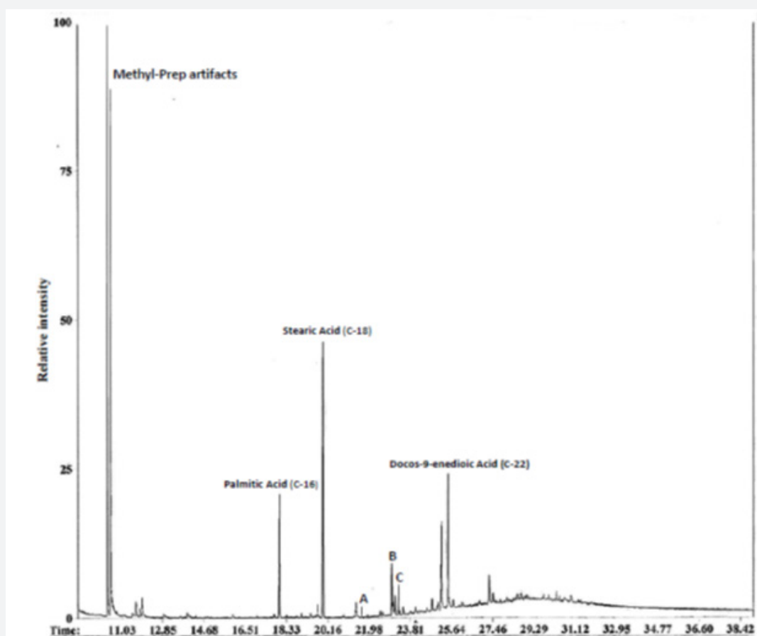
Figure 6: GC-MS chromatogram of lower chamber interior of ancient gourd-type double-chambered jar (sample no. 6A), El Diezmo-Adonaí (Colima), grave 7, vessel no. 6. Compounds A-C are (A) C 20 fatty acid; (B) C 22 alcohol; and (C) C 22 fatty acid. Note the absence of sterols and sapotenins at retention times between 29 and 31 minutes, as was observed for the modern replica jars (Figures 2 and 3). The large peaks at the start of the chromatogram are due to derivatization by Alltech II Me-Prep. The relative abundance of the total ion chromatograph is shown as a percentage on the ordinate..
