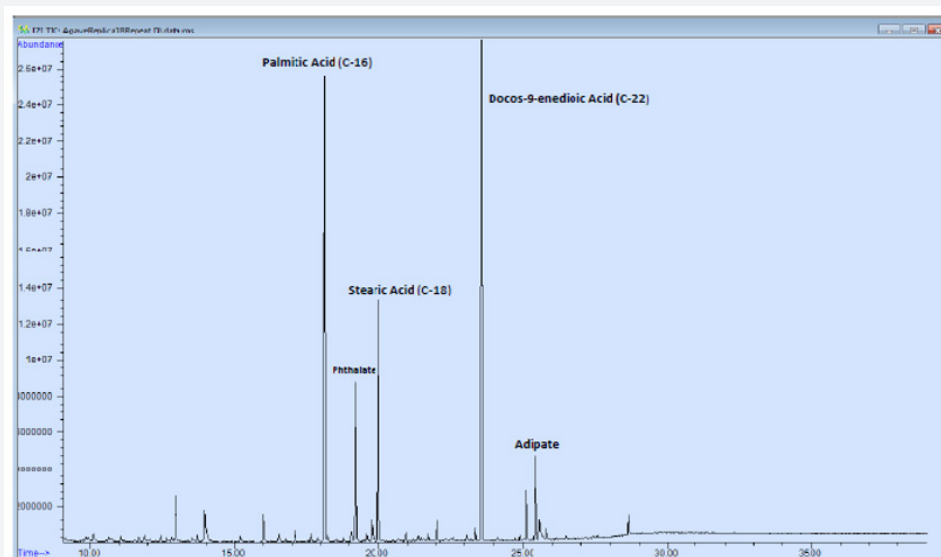
Figure 5: GC-MS chromatogram of modern replica of bowl exterior (sample no. 18). Ion abundance of the total ion chromatogram (TIC) is shown on the ordinate and retention time on the abscissa. e+ denotes an exponential.
