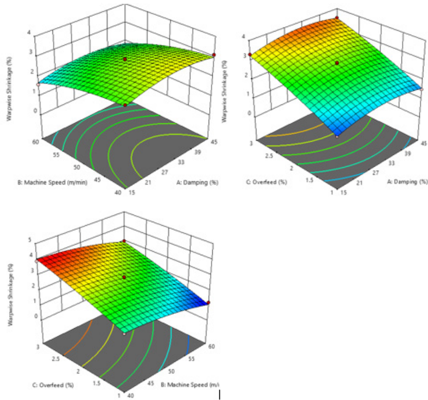
Figure 4: 3D surface plot showing the interactive effect of (a) damping % and machine speed (b) damping% and overfeed% (c) machine speed and overfeed% on warpwise shrinkage.
