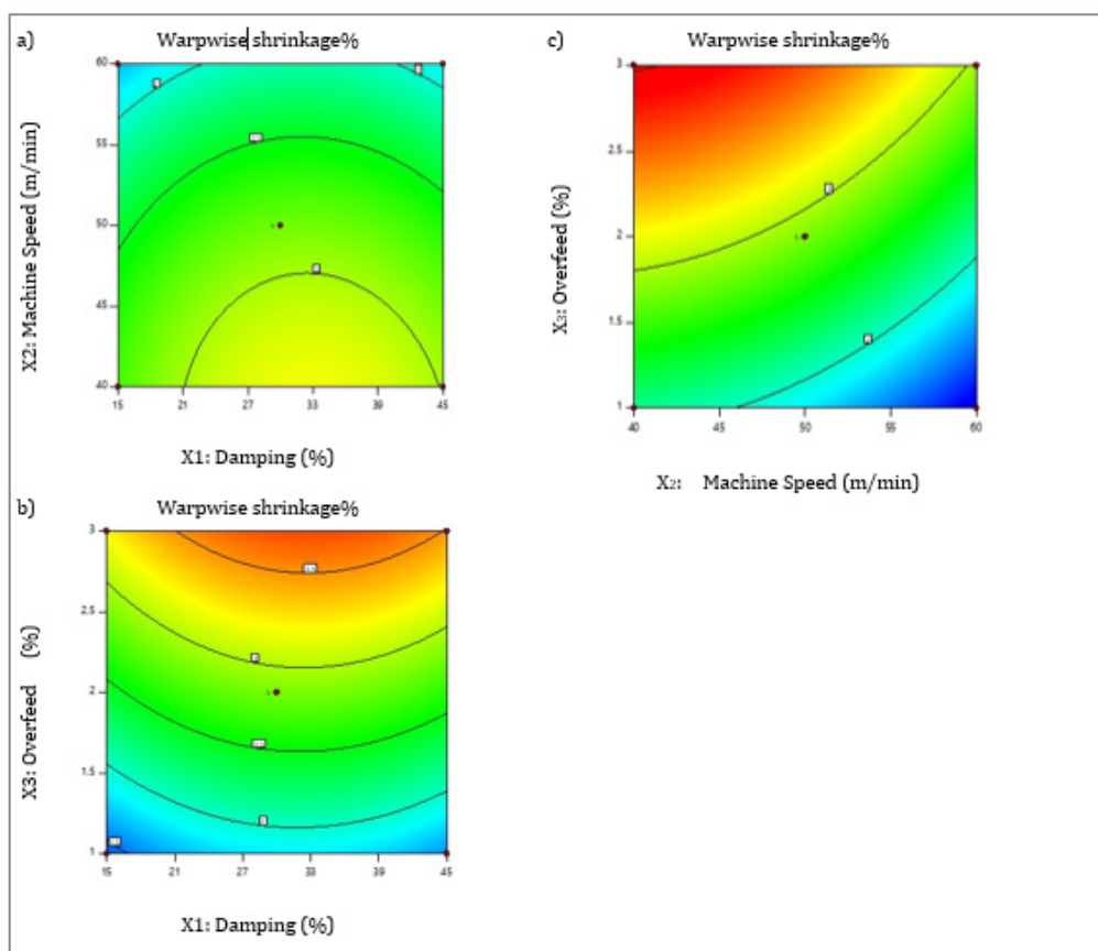
Figure 2: Contour plot showing the interactive effect of (a) damping % and machine speed (b) damping% and overfeed% (c) machine speed and overfeed% on warpwise shrinkage.
