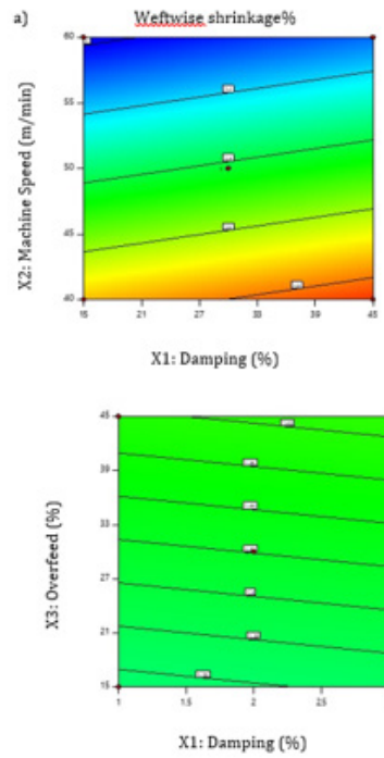
Figure 3: Contour plot showing the interactive effect of (a) damping % and machine speed (b) damping% and overfeed% on weftwise shrinkage.
