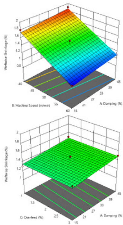
Figure 5: 3D surface plot showing the interactive effect of (a) damping % and machine speed (b) damping% and overfeed% on weftwise shrinkage.
