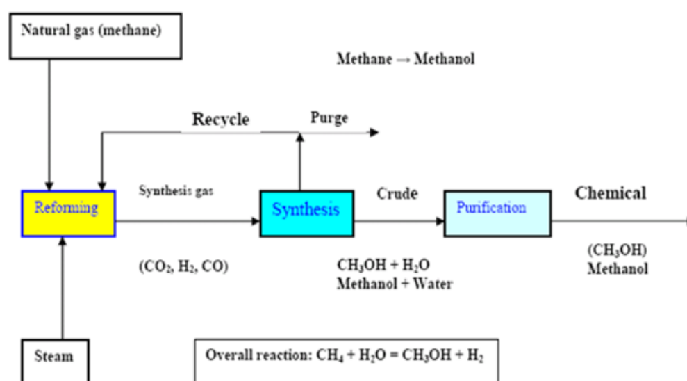
Figure 2: Schematic diagram shows methanol production [16].
