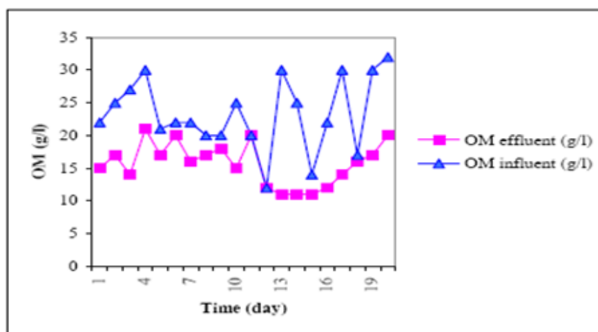
Figure 5: Organic matters before and after treatment in digester [29].
