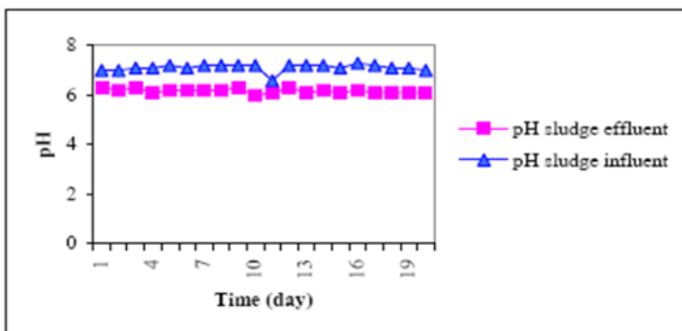
Figure 6: Potential of hydrogen (pH) sludge before and after treatment in the digester [29].
