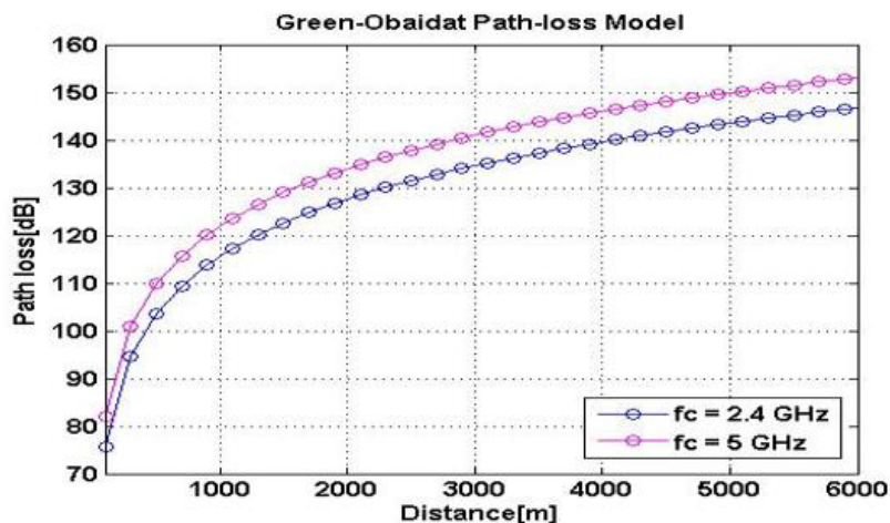
Figure 1: Green-Obaidat path-loss Model.
