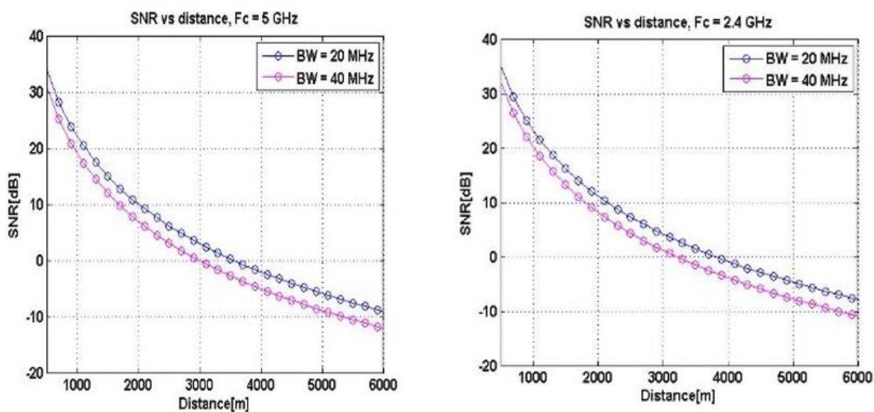
Figure 2: Variation of SNR with increasing distances a) F_c = 2.4 \text{ GHz} b) F_c = 05\text{GHz} .
