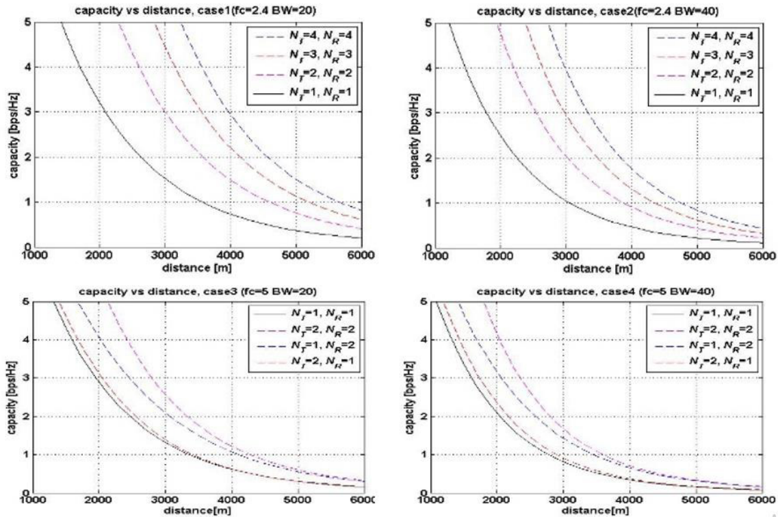
Figure 3: Capacity vs. distance for SISO and MIMO antenna system for a) Case 1 b) Case 2 c) Case 3 d) Case 4.
