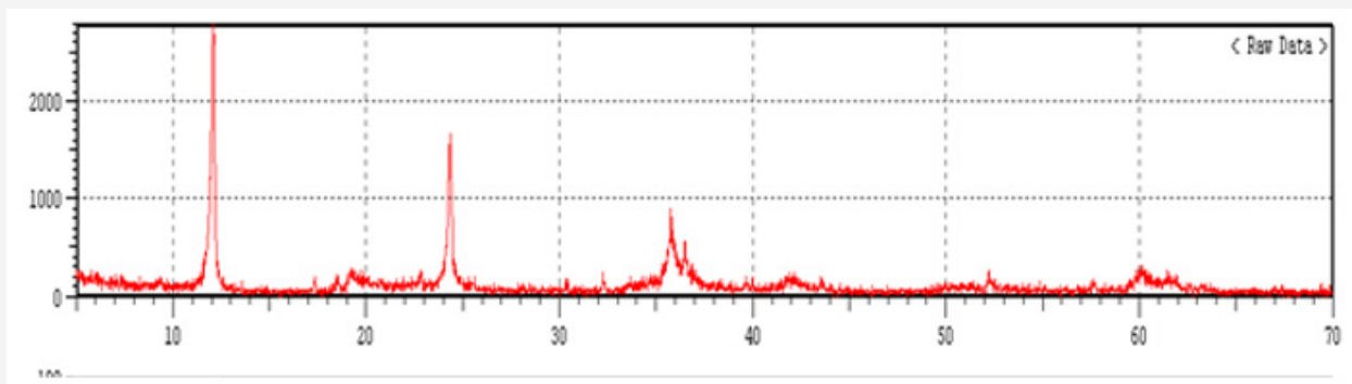
Figure 3: Diffractogram powder» of CFG «Saranovsky»: identified Lizardite-1T.
