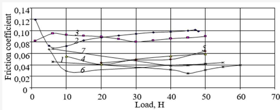
Figure 4: Friction coefficients steel tribological pair «finger-disk» in the motor oil Mobile SJ/SL API and 05W-30 SAE (1), as well as in motor mineral oil (2) and introduced in it tribological composition: preventive CAMP (3), serpentine CNT (4), MC-20 (5), «Saranovsky» (6) and nanodiamond KARAT (7).
