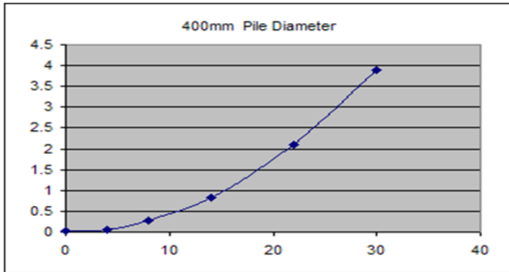
Figure 4: Typical Plot of Pile Load vs Depth for Pile Diameters of 400mm.
