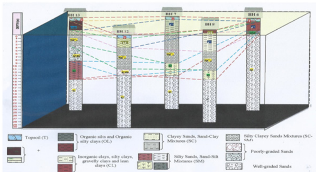
Figure 5b: Schematic Fence Diagram showing the Borings in Zone B.
