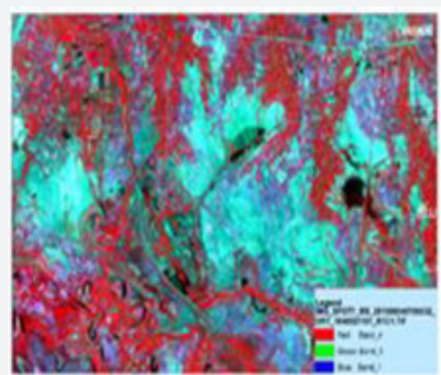
Figure 4: 4,3,1 channels combination (AZERSKY).
