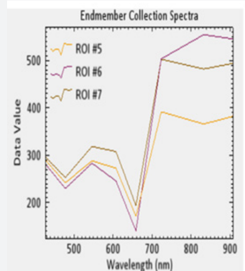
Figure 11: A generalized spectral curve of vegetation cover on saline soils.
