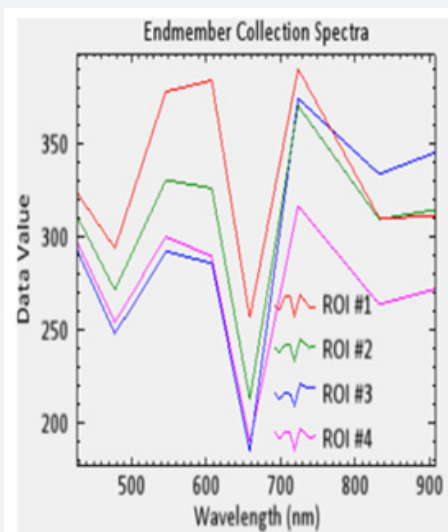
Figure 10: Generalized diagram of the spectral curves of soils with varying degrees of salinity.
